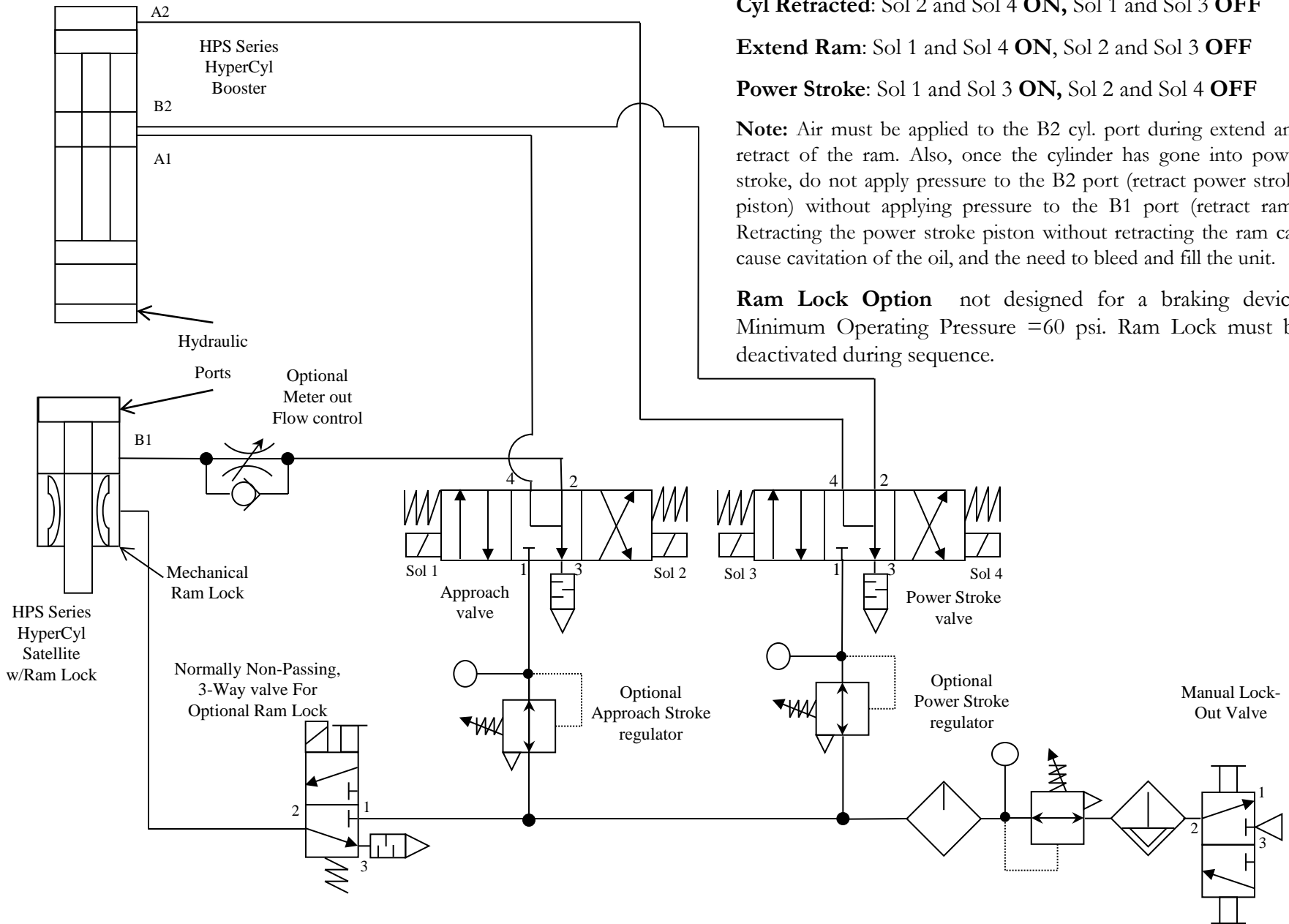
HPS 3-Position Open Center with Ram Lock Schematic
